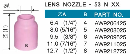
LENS NOZZLE - 53 N XX
