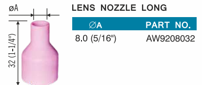
LENS NOZZLE LONG 53 N XX L
