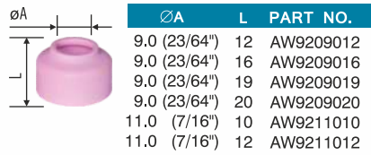
LENS NOZZLE - SHORT
